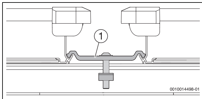
Fig. 43 Tensor bilateral del colector
