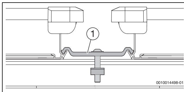
Fig. 50 Tensor bilateral del colector
