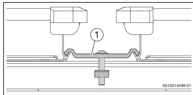
Fig. 55 Tensor bilateral del colector
