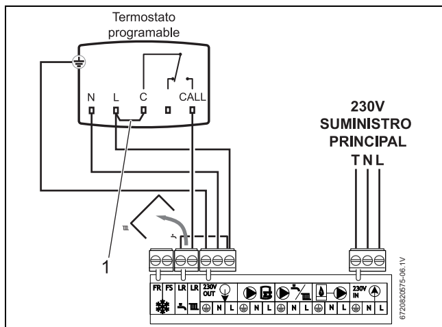
Fig. 61 Termostato programable
